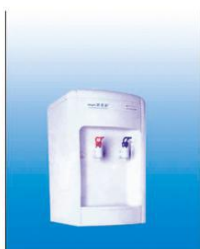
饮水机 Drinking Water Machine 300Lx300Wx500Hmm
